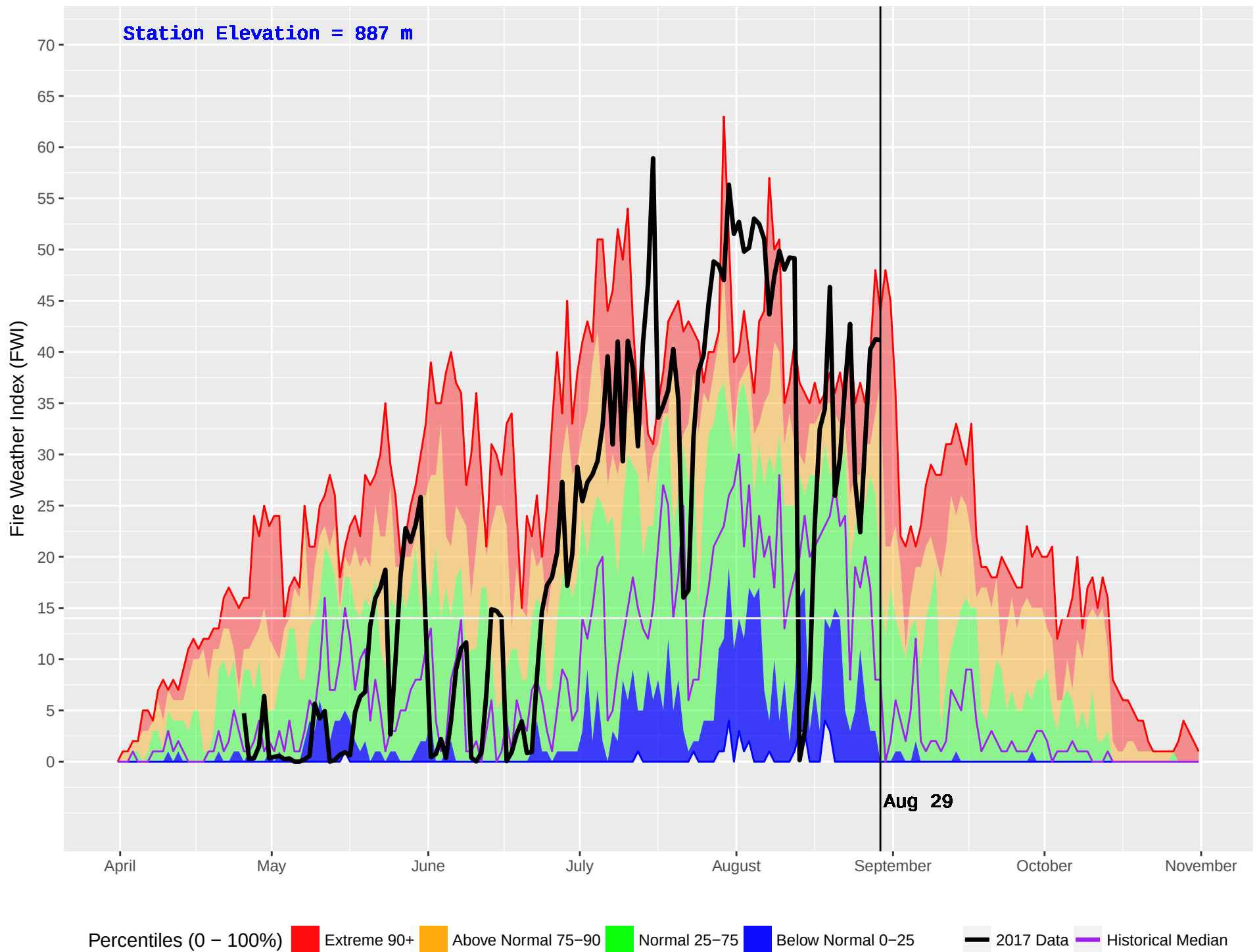
CRAWFORD (873) : Historical (2004–2016) and Current (2017) Noon Fire Weather Index (FWI)
