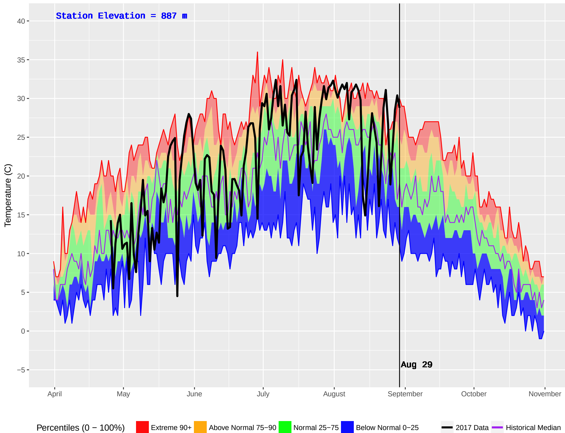
CRAWFORD (873) : Historical (2004–2016) and Current (2017) Noon Temperature
