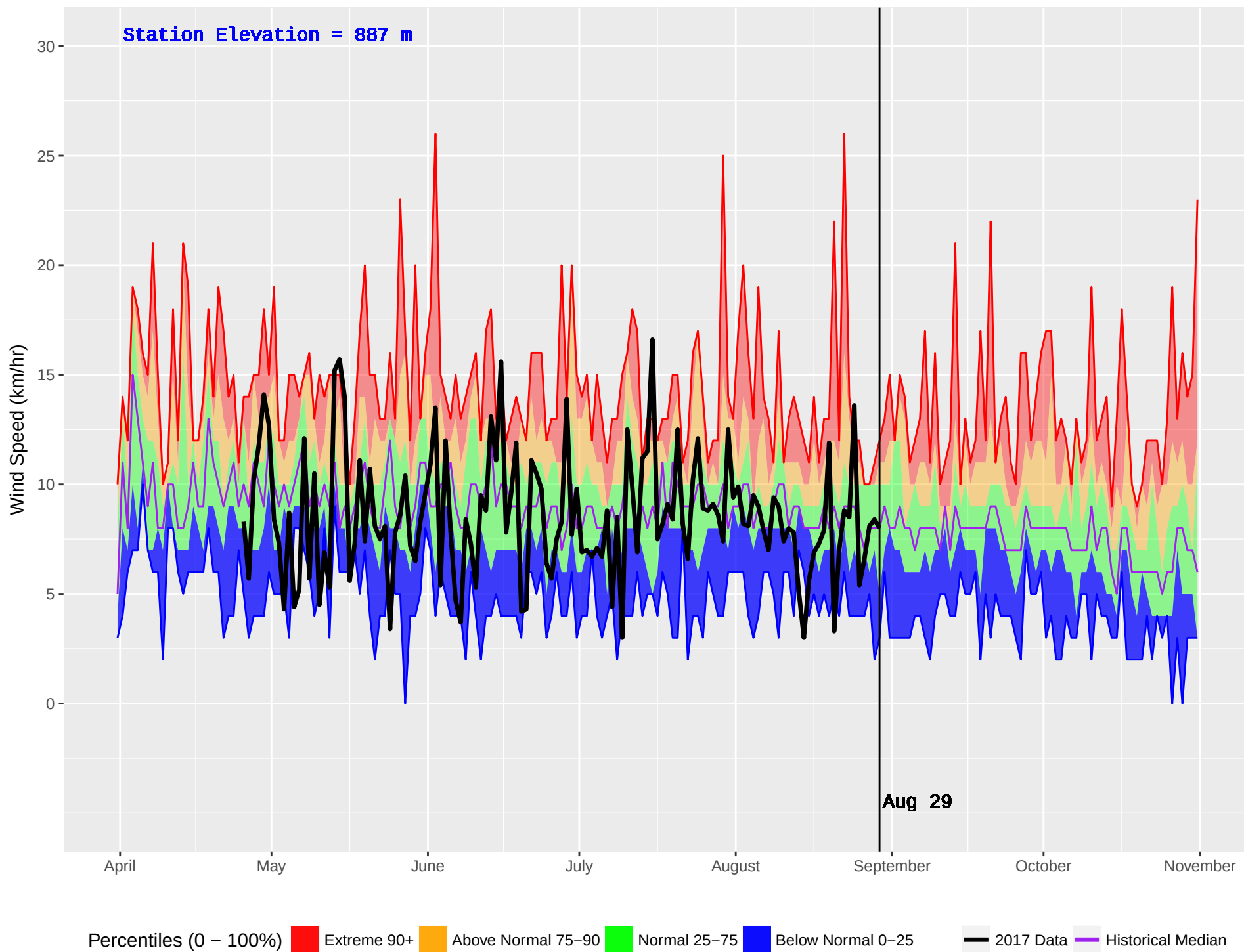
CRAWFORD (873) : Historical (2004–2016) and Current (2017) Noon Wind Speed
