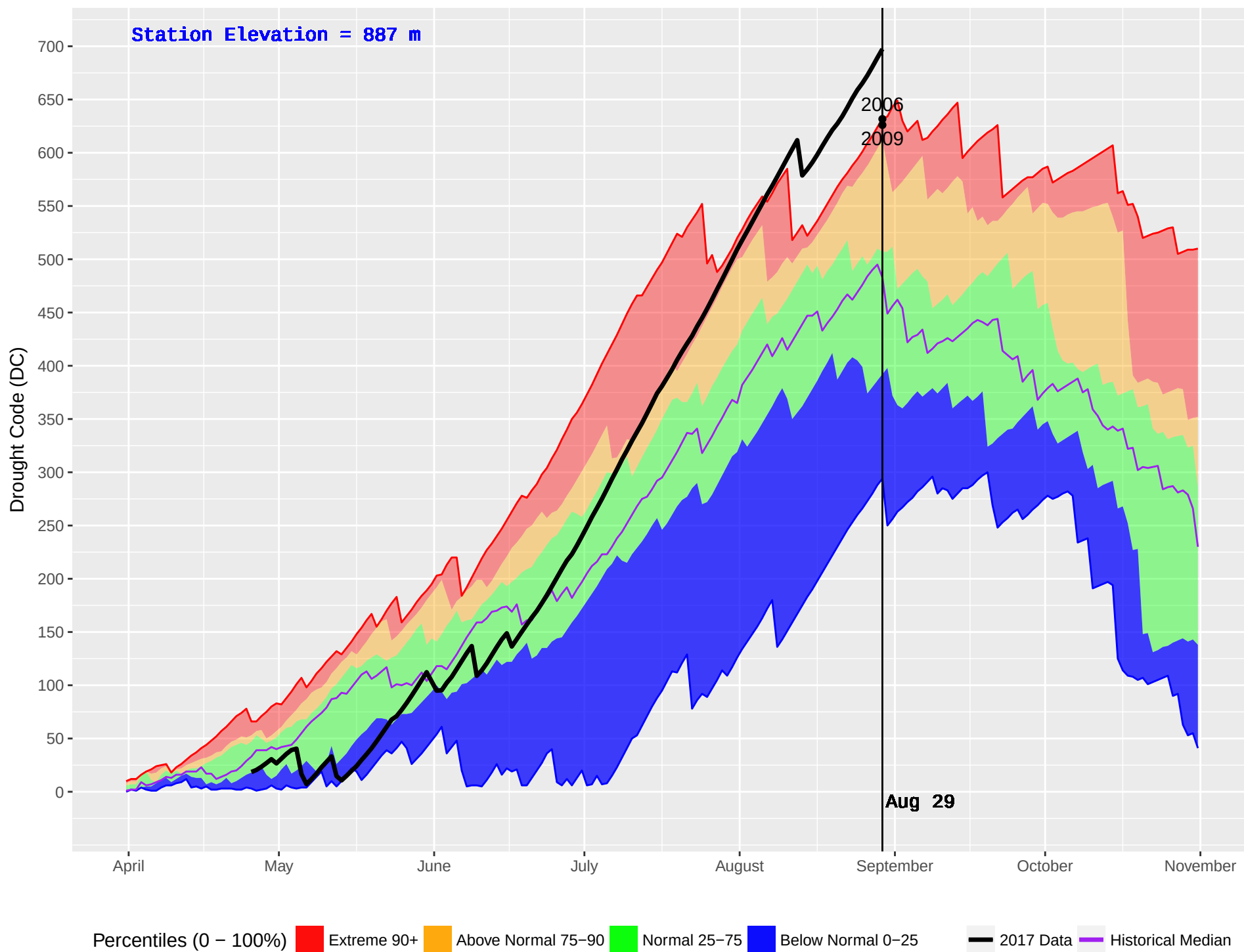
CRAWFORD (873) : Historical (2004–2016) and Current (2017) Noon Drought Code (DC)
