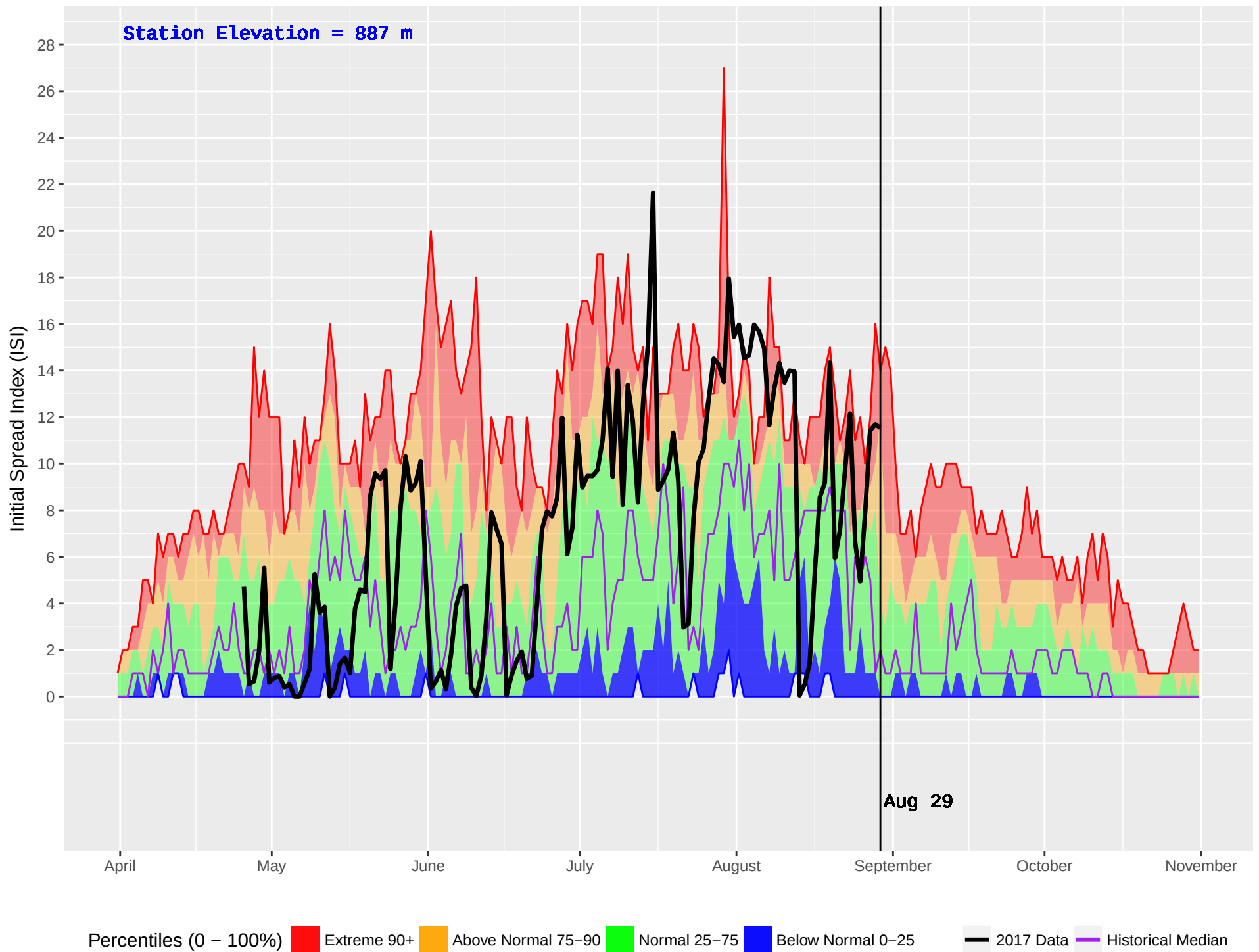
CRAWFORD (873) : Historical (2004–2016) and Current (2017) Noon Initial Spread Index (ISI)
